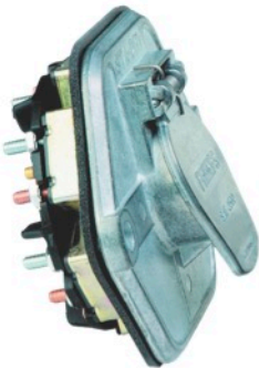
7 POLE SOCKET 20AMP C/B
